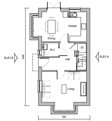
Ground Floor Plan Plots 4 & 11 Plots (handed) 1
