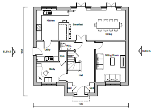
Ground Floor Plan Plots 7, 8 and 29 (handed)
