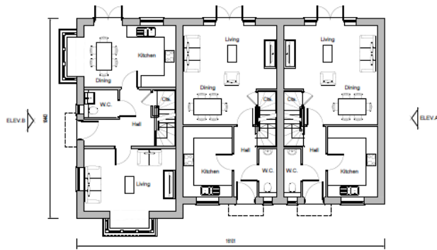
Ground Floor Plan Plots 78-80
